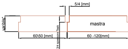
STANDARD TYPE OF MAST - TYPICAL SECTION
