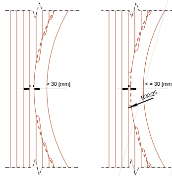
DEFINITION OF SHAPE IN CASE OF INTERSECTION BETWEEN CURVED SLATS AND MASTS
